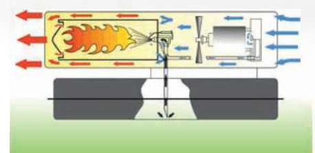
Combustion system - air flow
